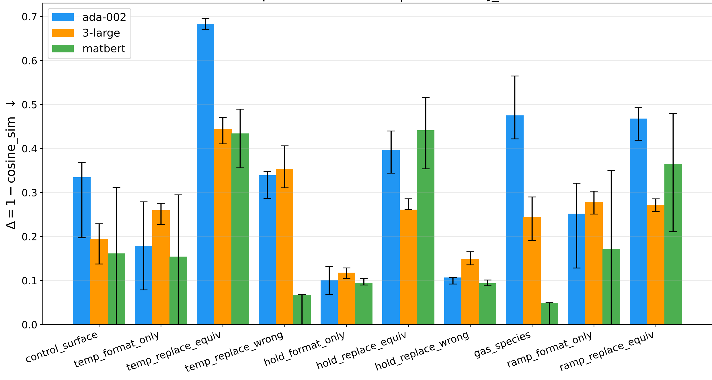
Group mean \Delta with IQR | Mode: PROJ_ref2
